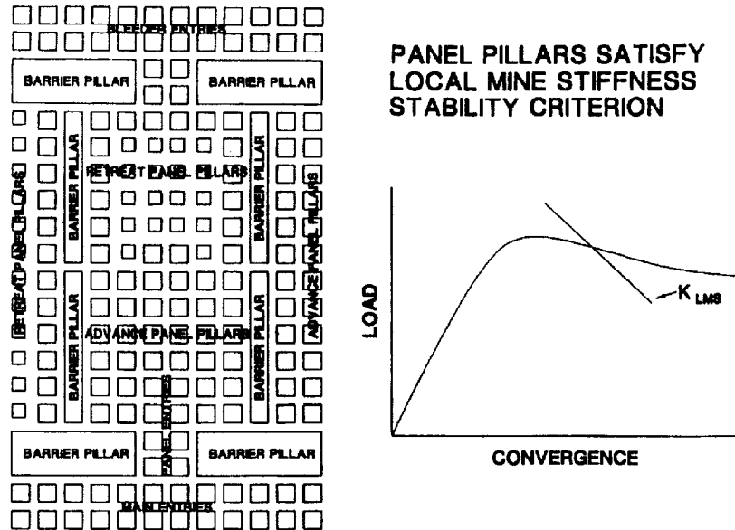
Fig. 5 Prevention approach: (a) unstable pillar failure is impossible because of either adequate stability factors (greater than 2) or high W/H ratios of panel pillars; (b) stability condition is such that high W/H -ratio panel pillars satisfy local mine stiffness stability criterion and CPF is physically impossible. Extraction for layout shown is 63%
