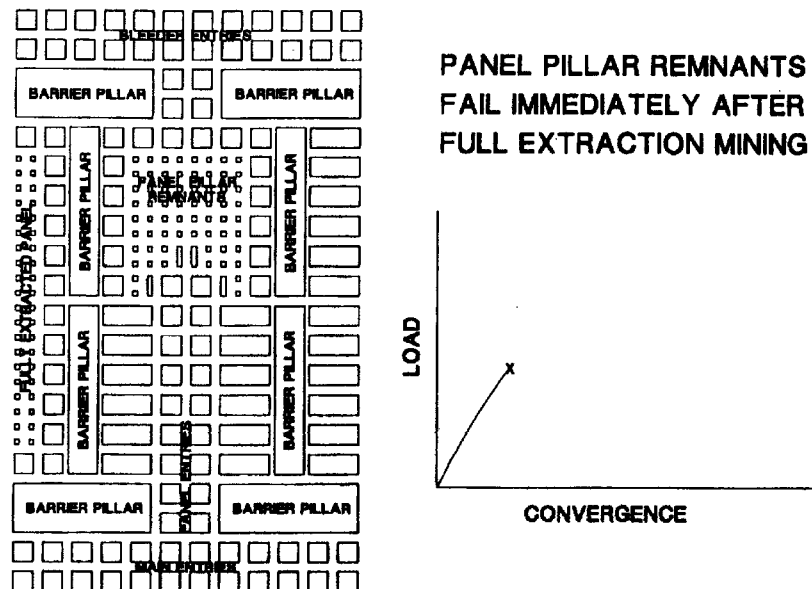
Fig. 6 Full extraction approach: (a) failure of pillar remnants along with overburden occurs immediately after pillar extraction; (b) retreat mining must ensure development of sufficiently weak remnant pillars. Extraction for layout shown is 67%
